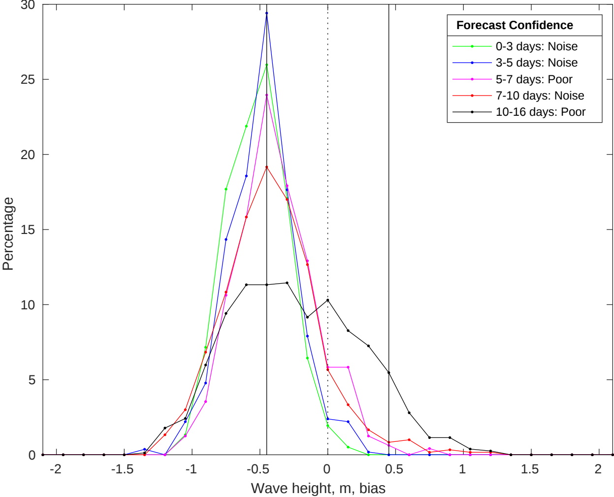
NDBC 46069 vs GFS Waves Bias Histogram: 06-Jul-2025
