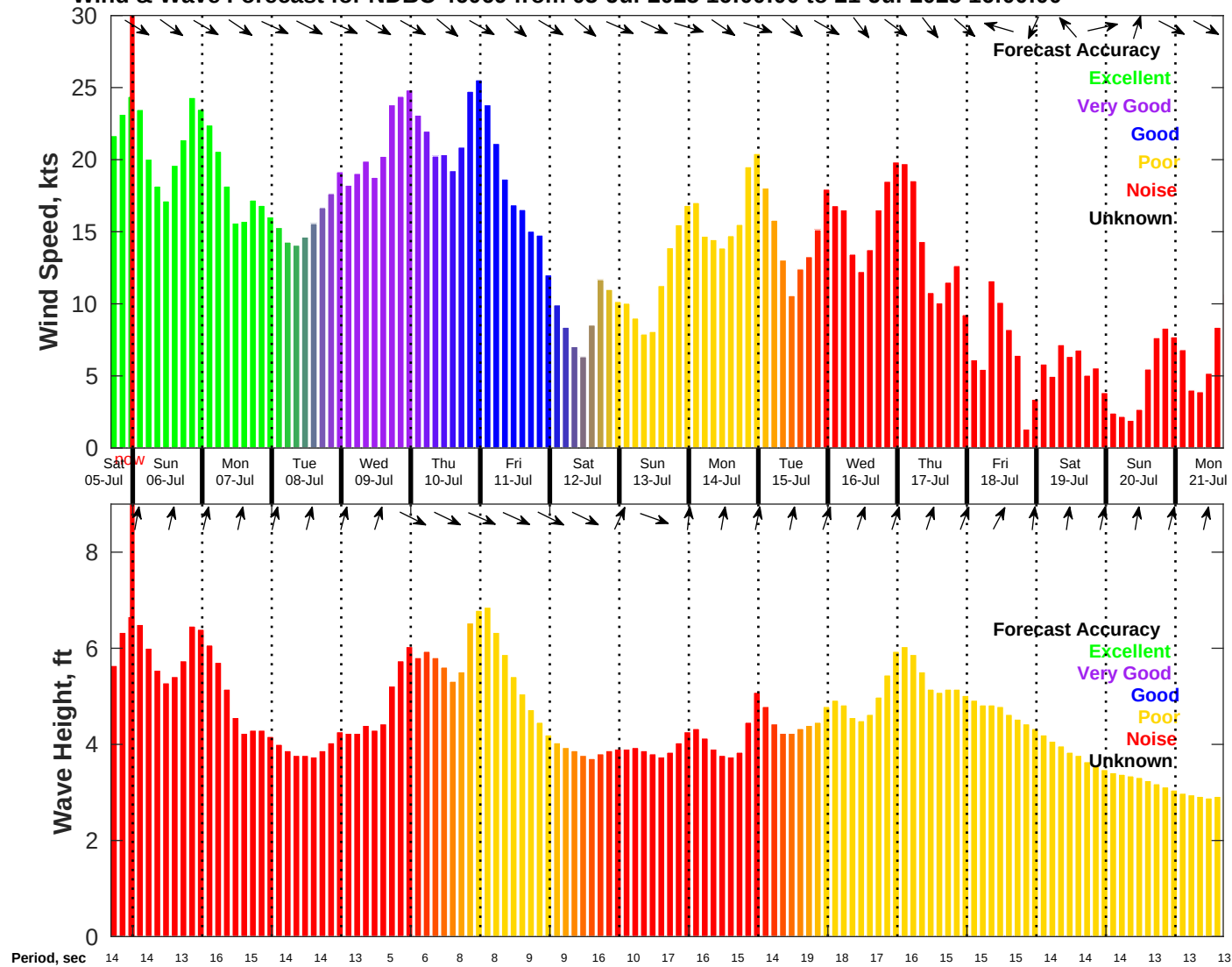
Wind & Wave Forecast for NDBC 46069 from 05-Jul-2025 16:00:00 to 21-Jul-2025 16:00:00
