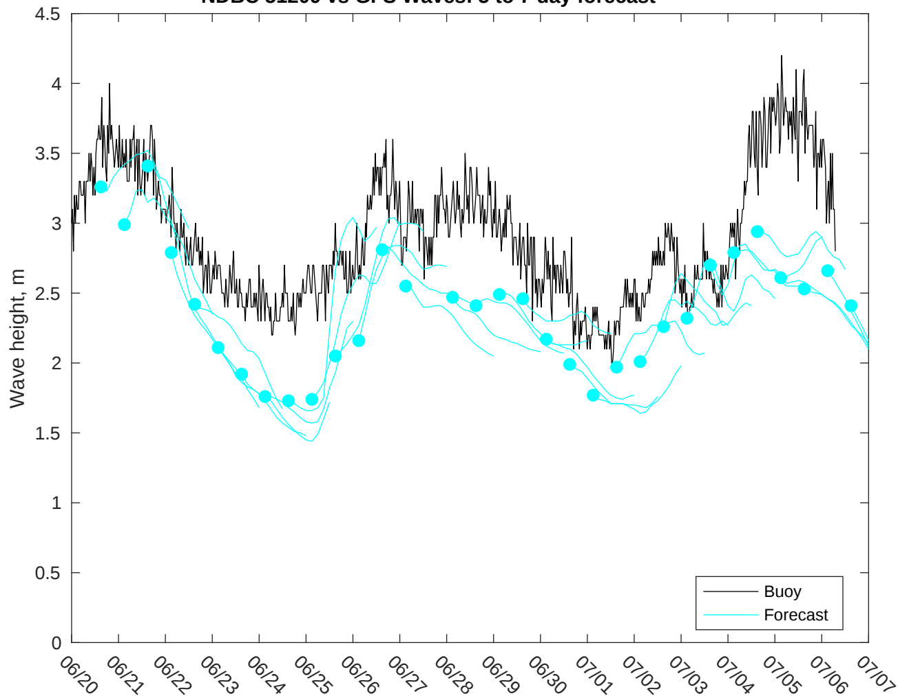
NDBC 51209 vs GFS Waves: 5 to 7 day forecast
