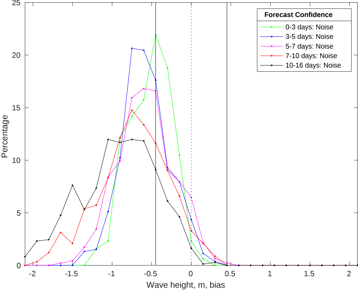
NDBC 51209 vs GFS Waves Bias Histogram: 06-Jul-2025
