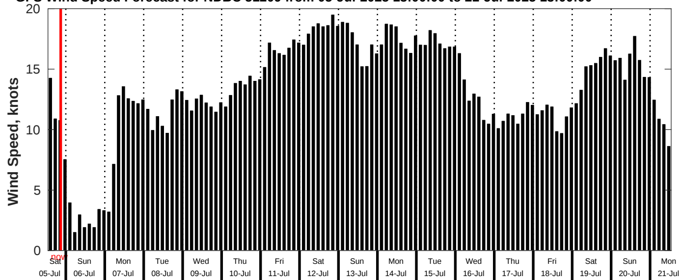
GFS Wind Speed Forecast for NDBC 51209 from 05-Jul-2025 13:00:00 to 21-Jul-2025 13:00:00
