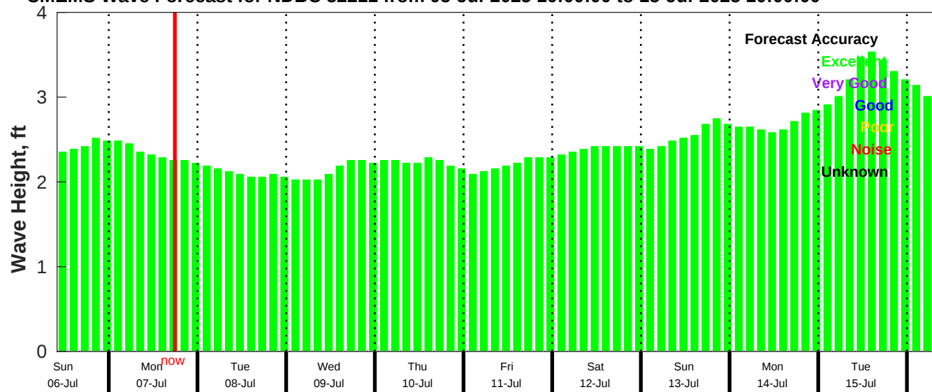
CMEMS Wave Forecast for NDBC 52211 from 05-Jul-2025 10:00:00 to 15-Jul-2025 10:00:00
