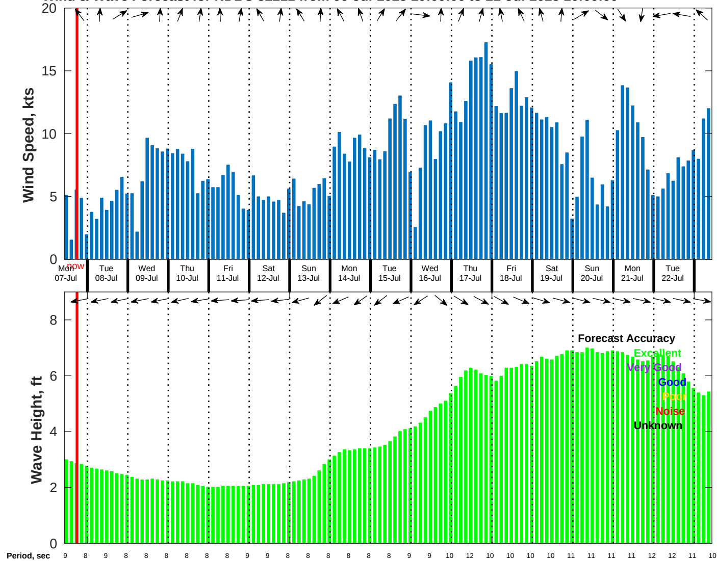
Wind & Wave Forecast for NDBC 52211 from 06-Jul-2025 10:00:00 to 22-Jul-2025 10:00:00
