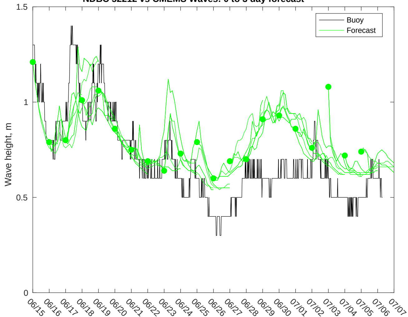
NDBC 52212 vs CMEMS Waves: 0 to 3 day forecast
