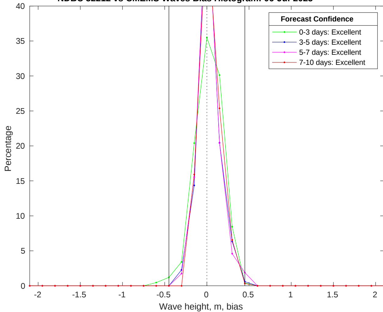
NDBC 52212 vs CMEMS Waves Bias Histogram: 06-Jul-2025
