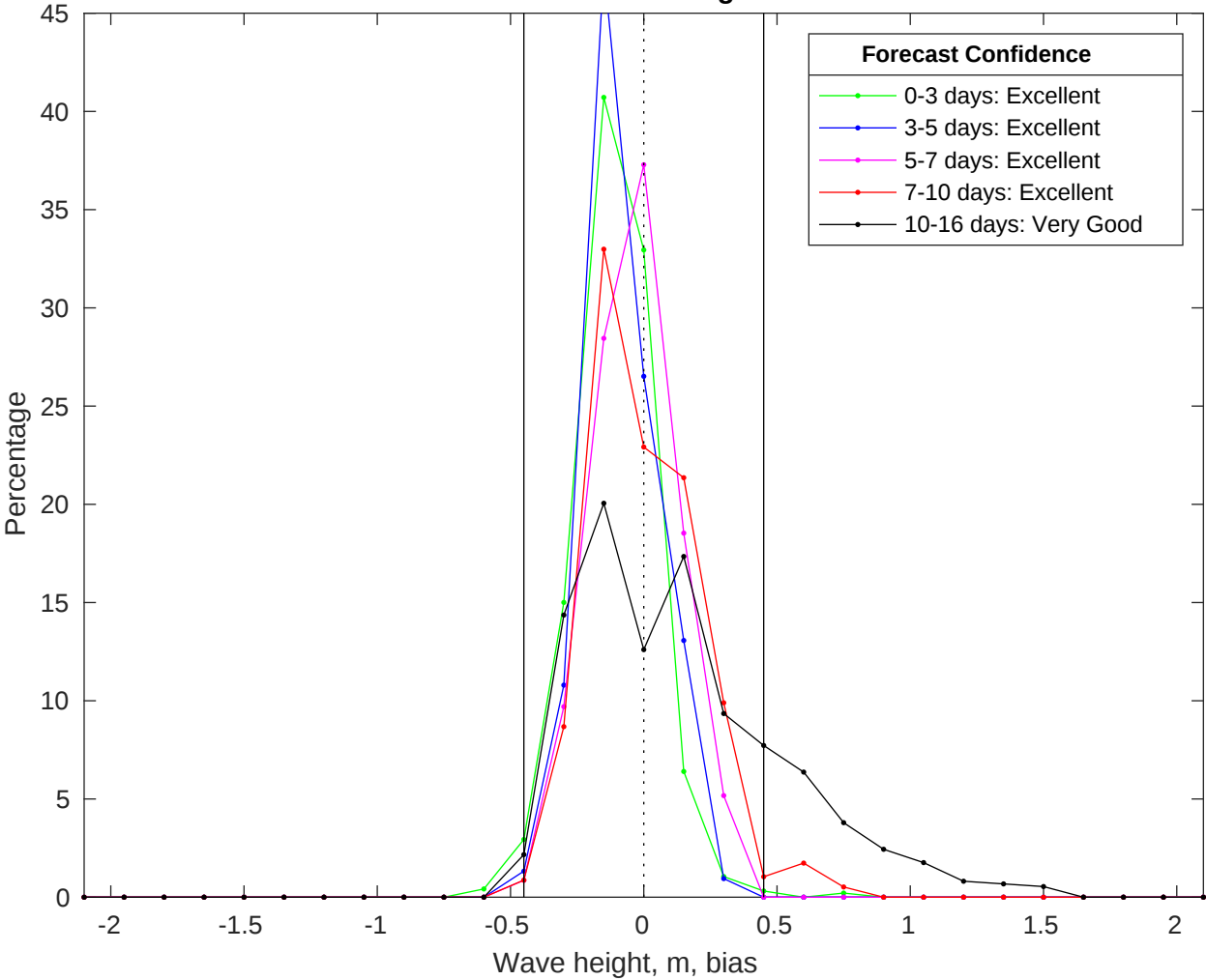
NDBC 52212 vs GFS Waves Bias Histogram: 06-Jul-2025
