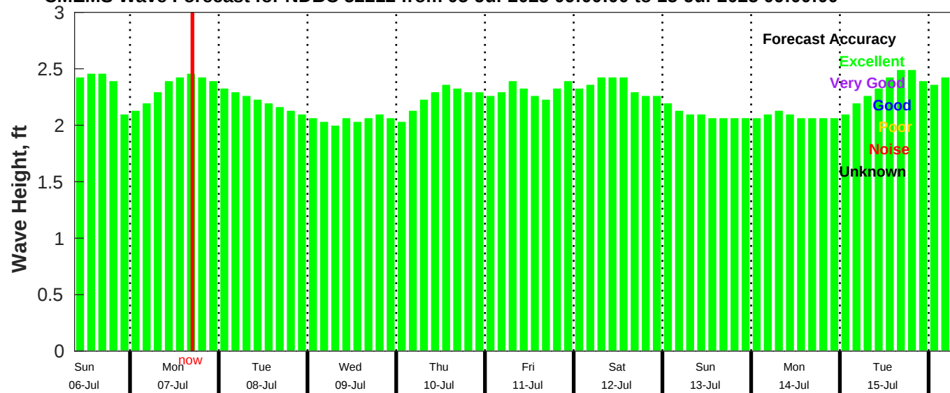
CMEMS Wave Forecast for NDBC 52212 from 05-Jul-2025 09:00:00 to 15-Jul-2025 09:00:00
