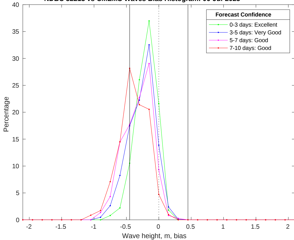
NDBC 52213 vs CMEMS Waves Bias Histogram: 06-Jul-2025
