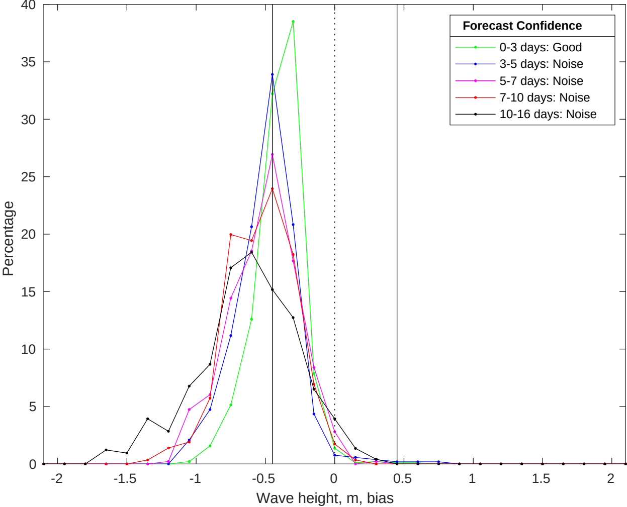
NDBC 52213 vs GFS Waves Bias Histogram: 06-Jul-2025
