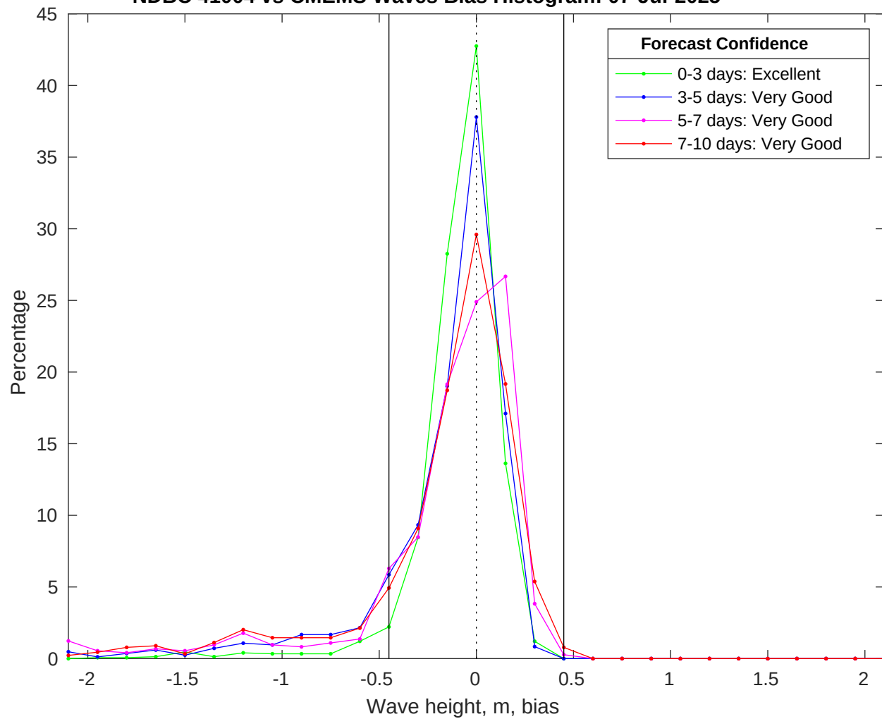
NDBC 41004 vs CMEMS Waves Bias Histogram: 07-Jul-2025
