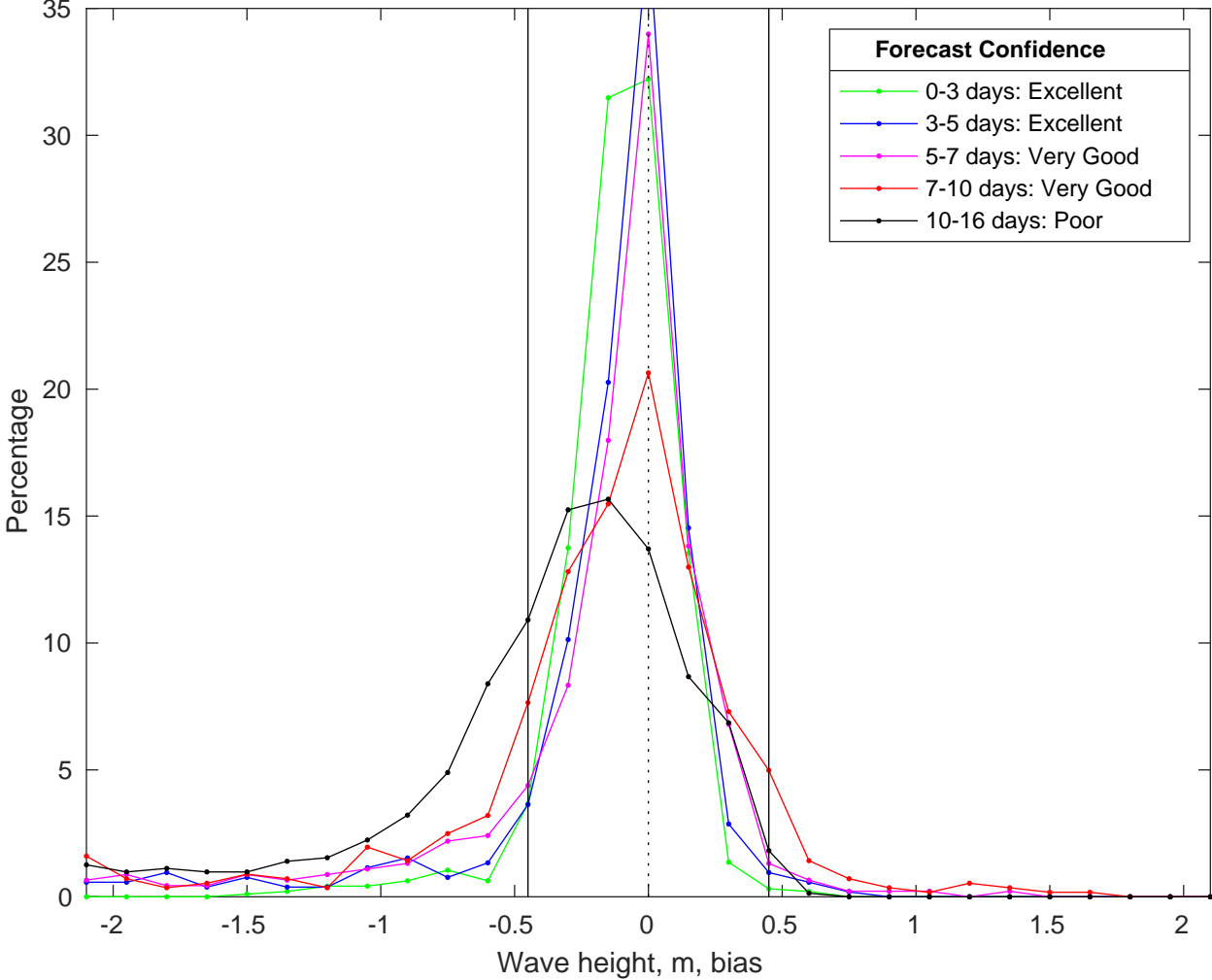
NDBC 41004 vs GFS Waves Bias Histogram: 07-Jul-2025
