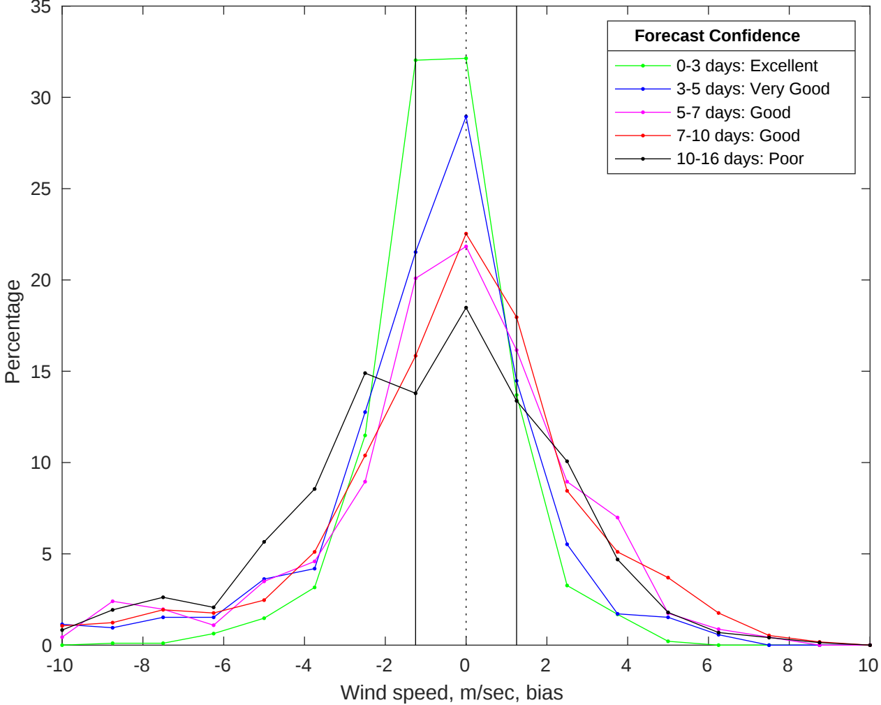
NDBC 41004 vs GFS Winds Bias Histogram: 07-Jul-2025
