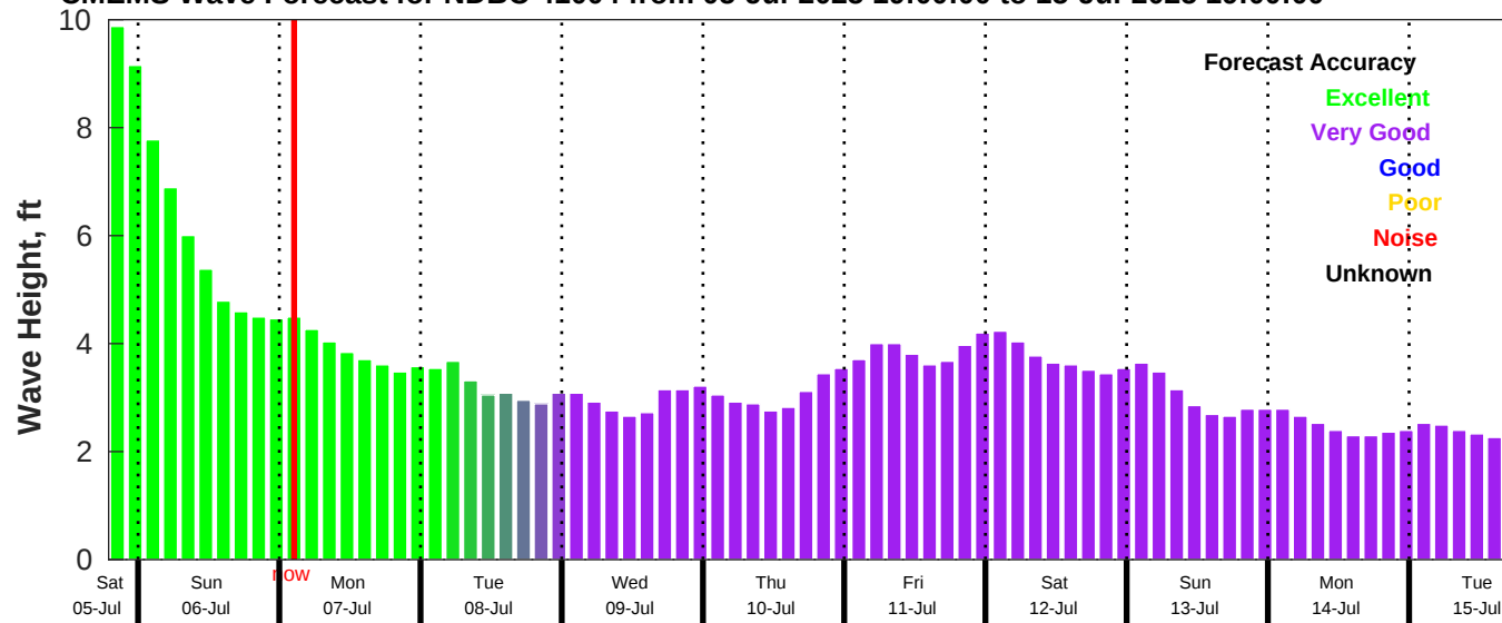
CMEMS Wave Forecast for NDBC 41004 from 05-Jul-2025 19:00:00 to 15-Jul-2025 19:00:00
