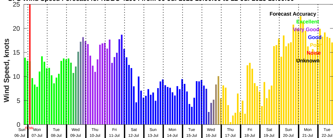
GFS Wind Speed Forecast for NDBC 41004 from 06-Jul-2025 19:00:00 to 22-Jul-2025 19:00:00
