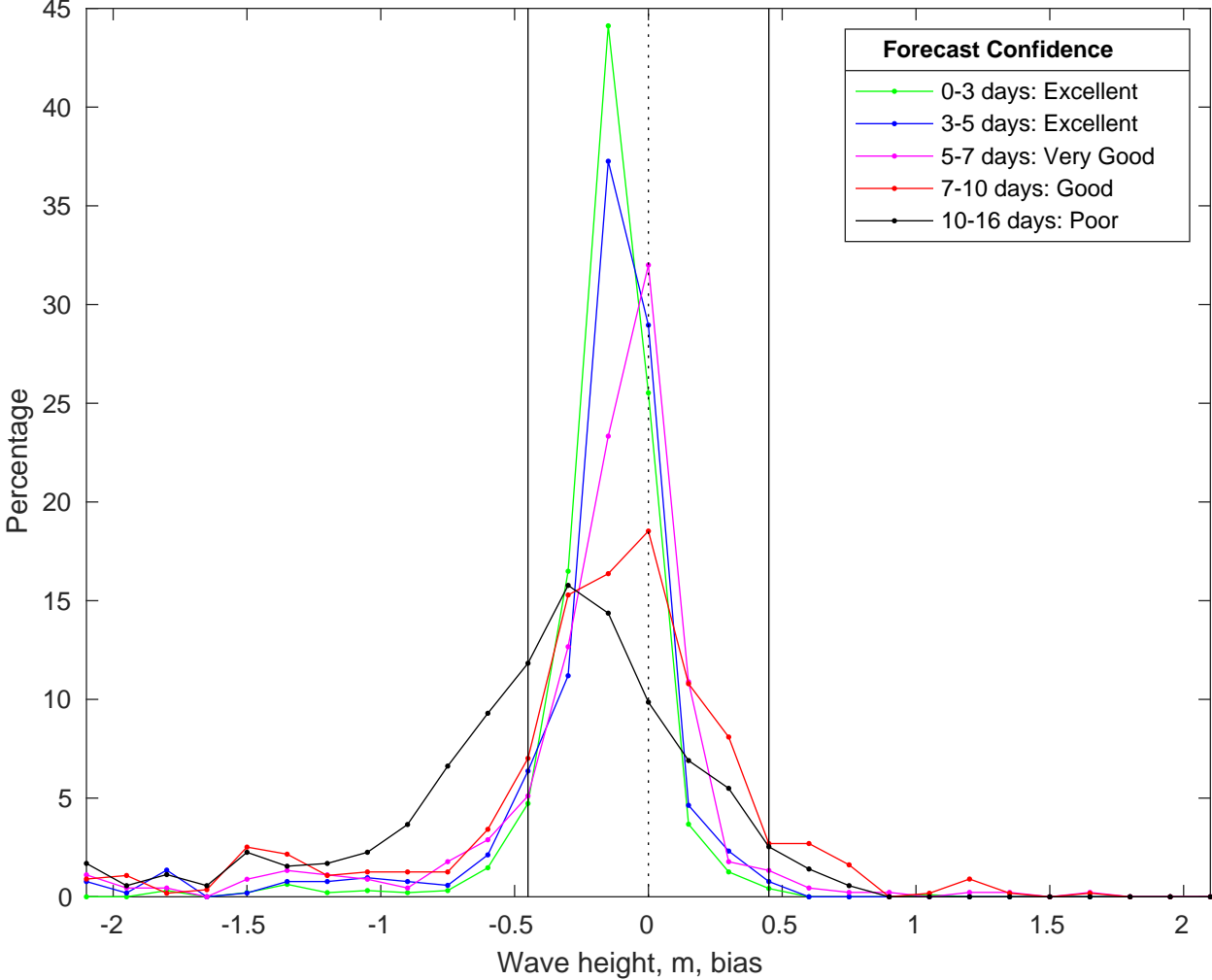
NDBC 41013 vs GFS Waves Bias Histogram: 07-Jul-2025
