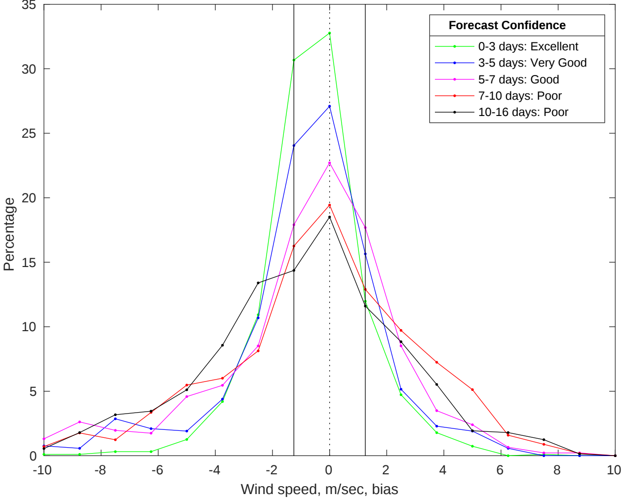
NDBC 41013 vs GFS Winds Bias Histogram: 07-Jul-2025
