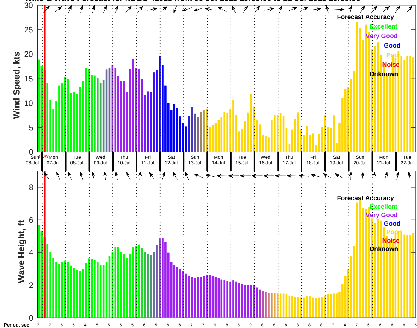
Wind & Wave Forecast for NDBC 41013 from 06-Jul-2025 19:00:00 to 22-Jul-2025 19:00:00
