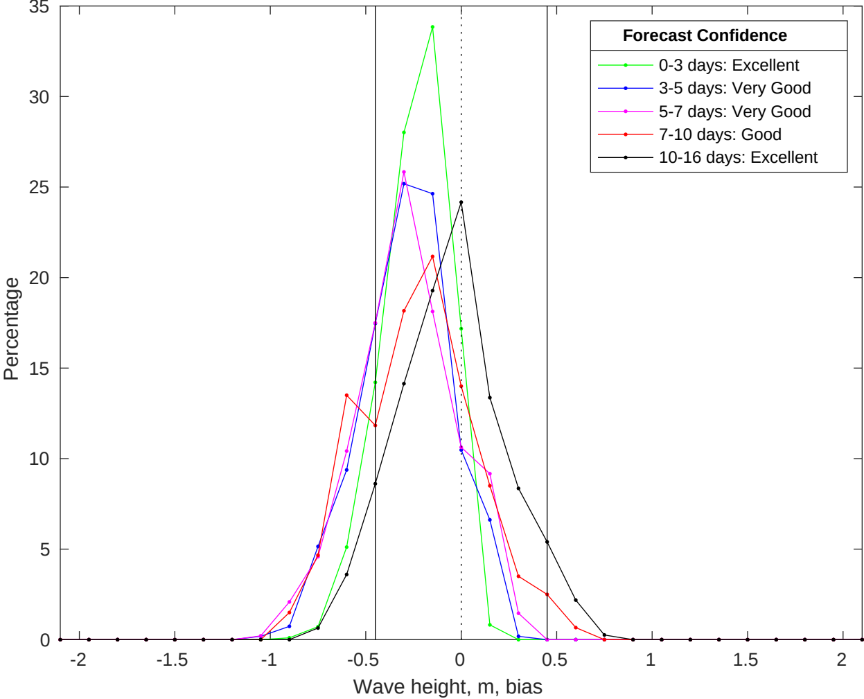
NDBC 41040 vs GFS Waves Bias Histogram: 07-Jul-2025
