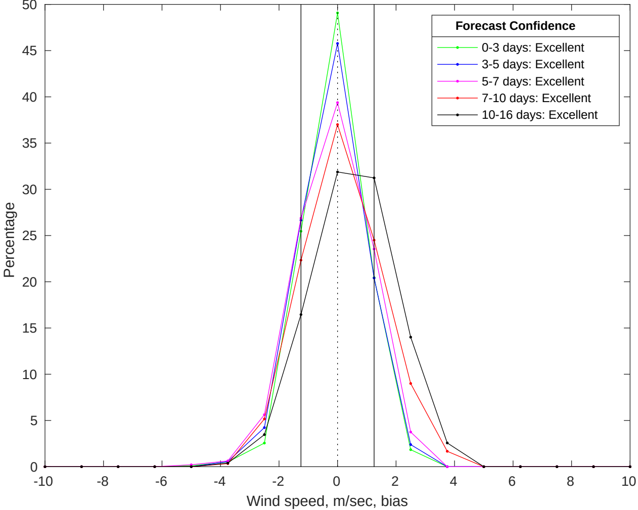
NDBC 41040 vs GFS Winds Bias Histogram: 07-Jul-2025
