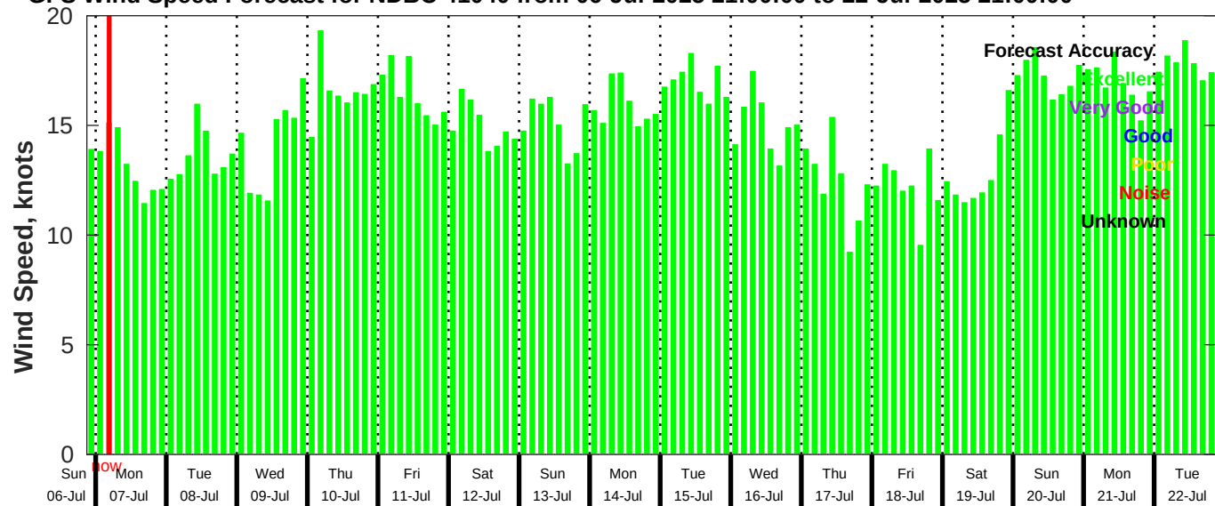
GFS Wind Speed Forecast for NDBC 41040 from 06-Jul-2025 21:00:00 to 22-Jul-2025 21:00:00
