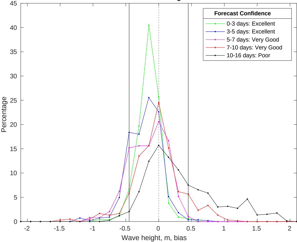
NDBC 42019 vs GFS Waves Bias Histogram: 07-Jul-2025
