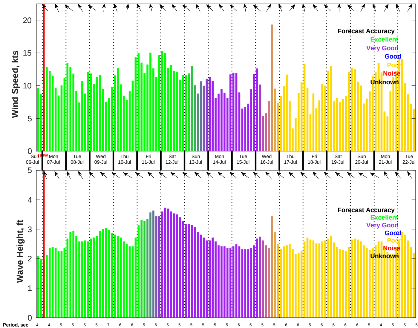
Wind & Wave Forecast for NDBC 42019 from 06-Jul-2025 18:00:00 to 22-Jul-2025 18:00:00
