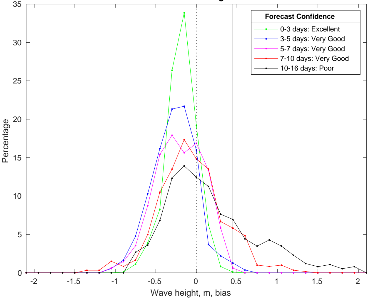
NDBC 42020 vs GFS Waves Bias Histogram: 07-Jul-2025
