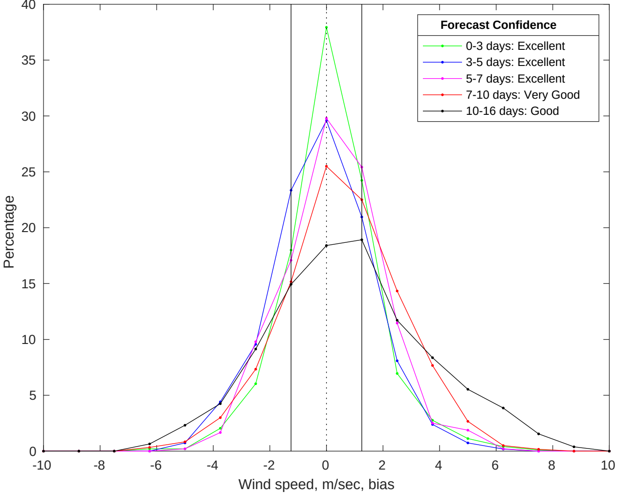
NDBC 42020 vs GFS Winds Bias Histogram: 07-Jul-2025
