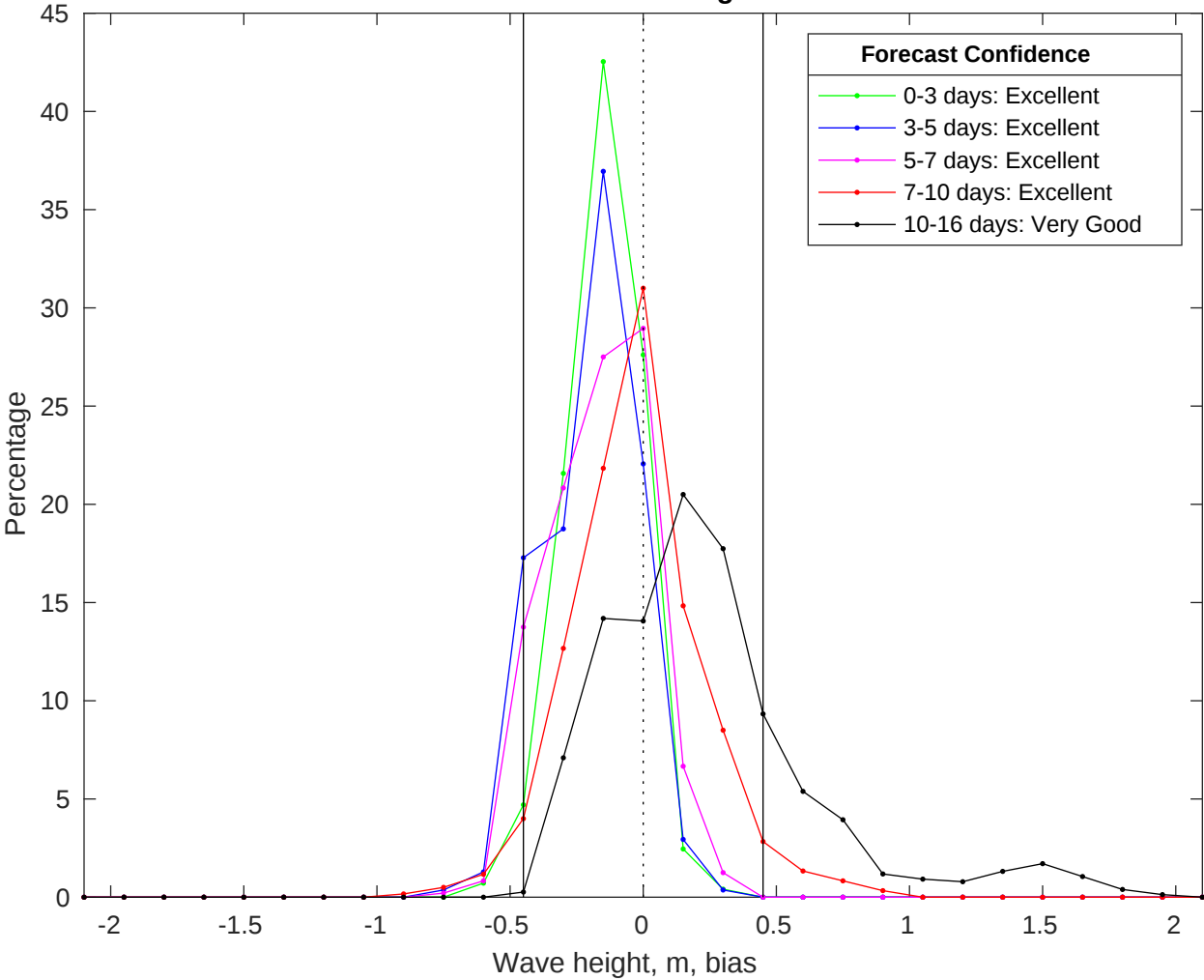
NDBC 42035 vs GFS Waves Bias Histogram: 07-Jul-2025
