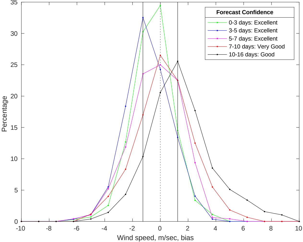
NDBC 42035 vs GFS Winds Bias Histogram: 07-Jul-2025
