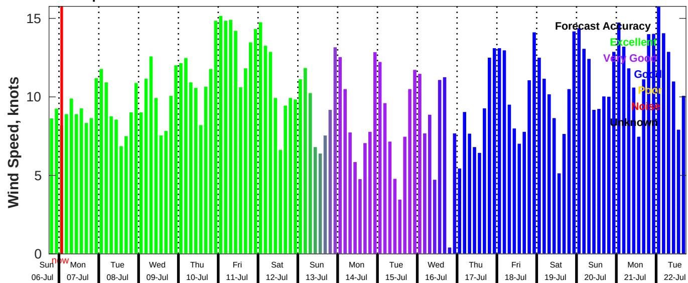
GFS Wind Speed Forecast for NDBC 42035 from 06-Jul-2025 18:00:00 to 22-Jul-2025 18:00:00
