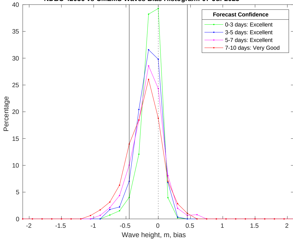
NDBC 42036 vs CMEMS Waves Bias Histogram: 07-Jul-2025
