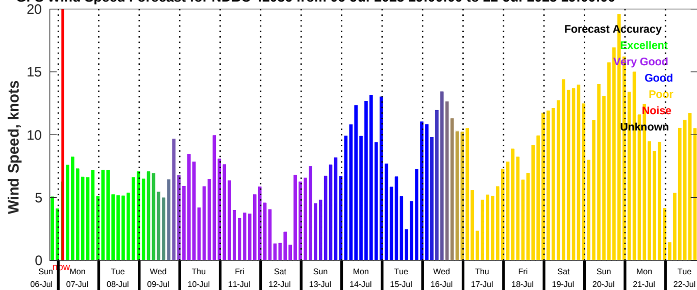
GFS Wind Speed Forecast for NDBC 42036 from 06-Jul-2025 19:00:00 to 22-Jul-2025 19:00:00
