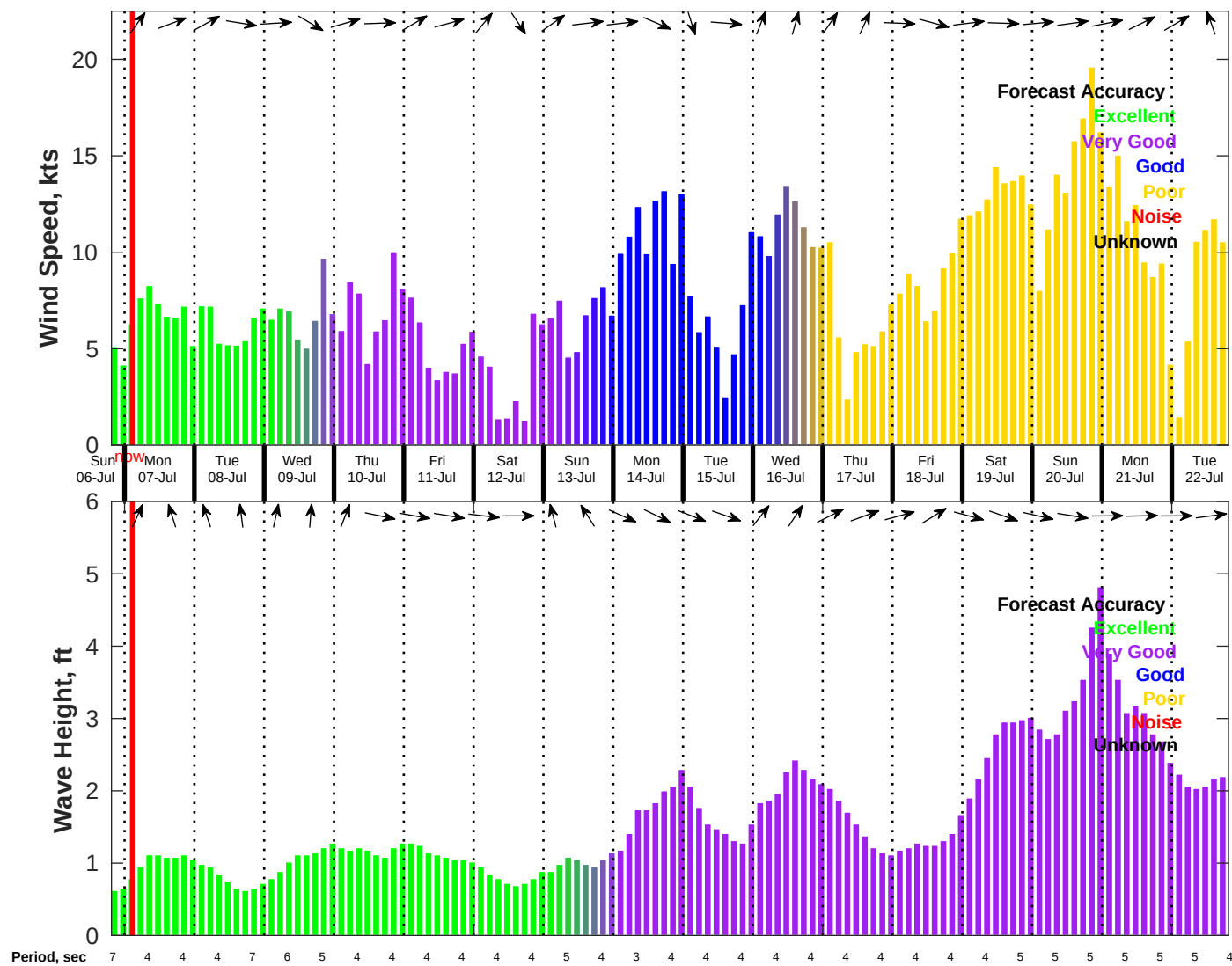
Wind & Wave Forecast for NDBC 42036 from 06-Jul-2025 19:00:00 to 22-Jul-2025 19:00:00
