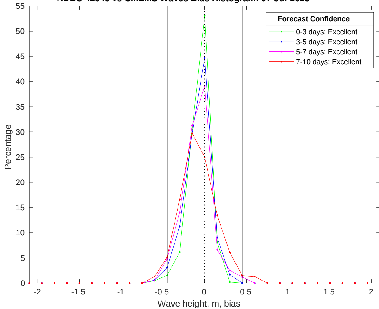
NDBC 42040 vs CMEMS Waves Bias Histogram: 07-Jul-2025
