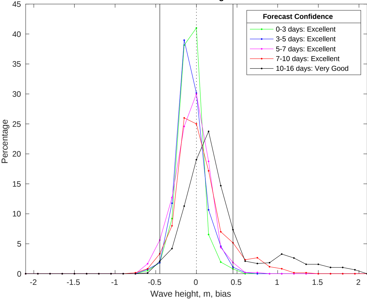
NDBC 42040 vs GFS Waves Bias Histogram: 07-Jul-2025
