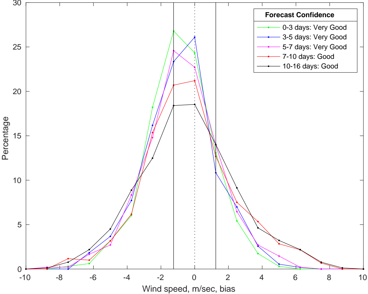
NDBC 42040 vs GFS Winds Bias Histogram: 07-Jul-2025
