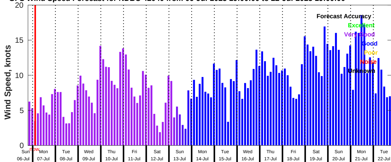
GFS Wind Speed Forecast for NDBC 42040 from 06-Jul-2025 19:00:00 to 22-Jul-2025 19:00:00
