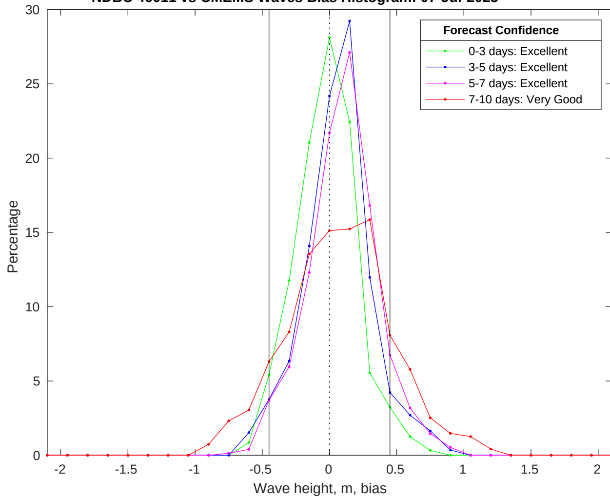
NDBC 46011 vs CMEMS Waves Bias Histogram: 07-Jul-2025
