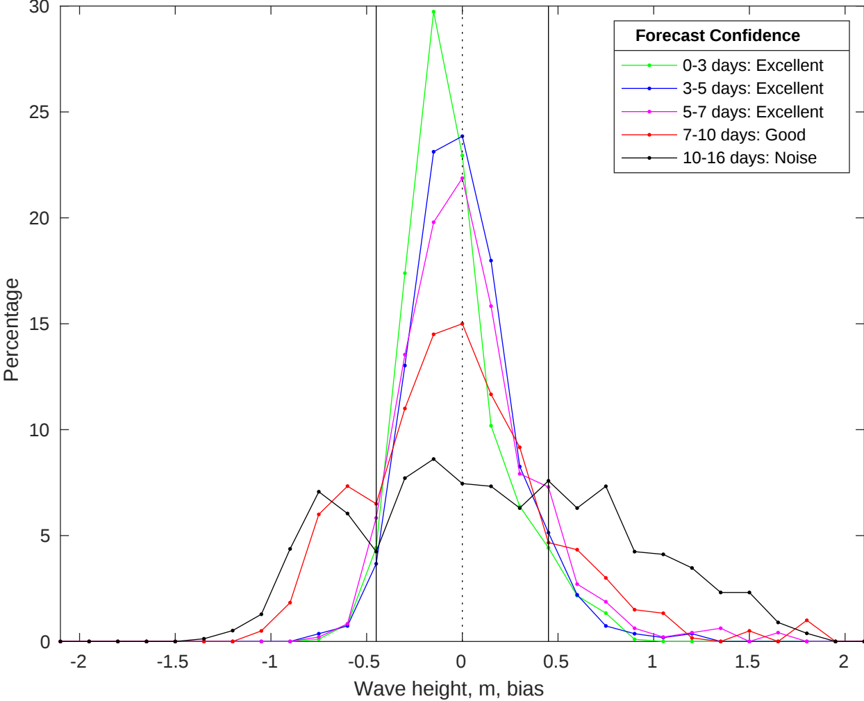
NDBC 46011 vs GFS Waves Bias Histogram: 07-Jul-2025
