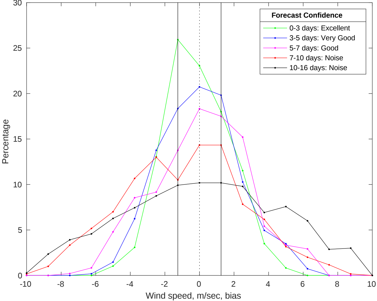
NDBC 46011 vs GFS Winds Bias Histogram: 07-Jul-2025
