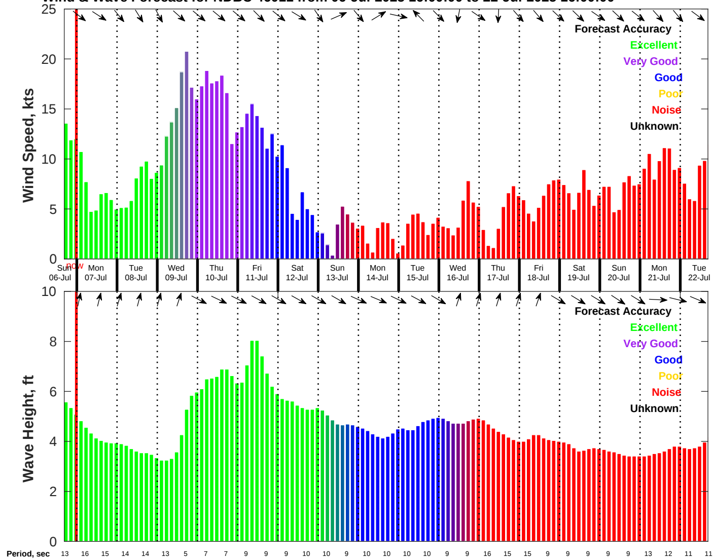
Wind & Wave Forecast for NDBC 46011 from 06-Jul-2025 16:00:00 to 22-Jul-2025 16:00:00
