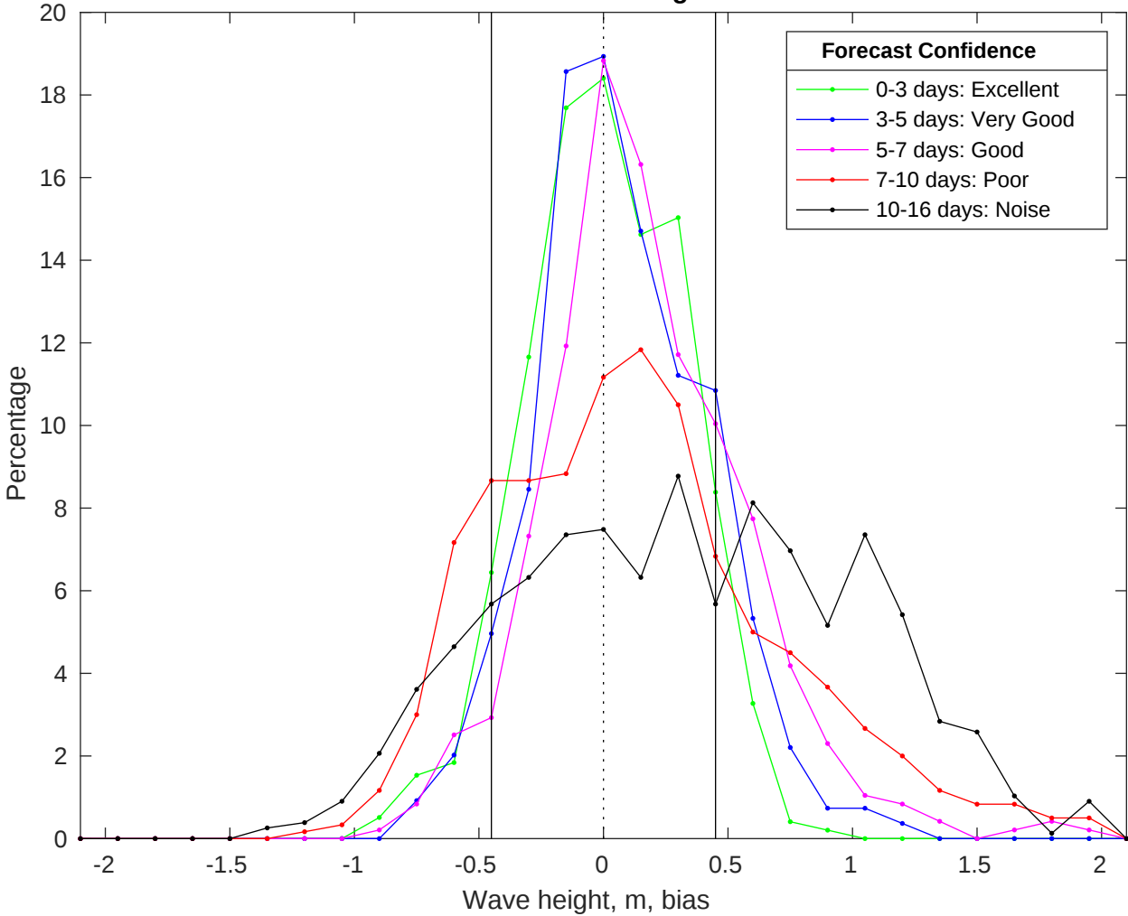
NDBC 46028 vs GFS Waves Bias Histogram: 07-Jul-2025
