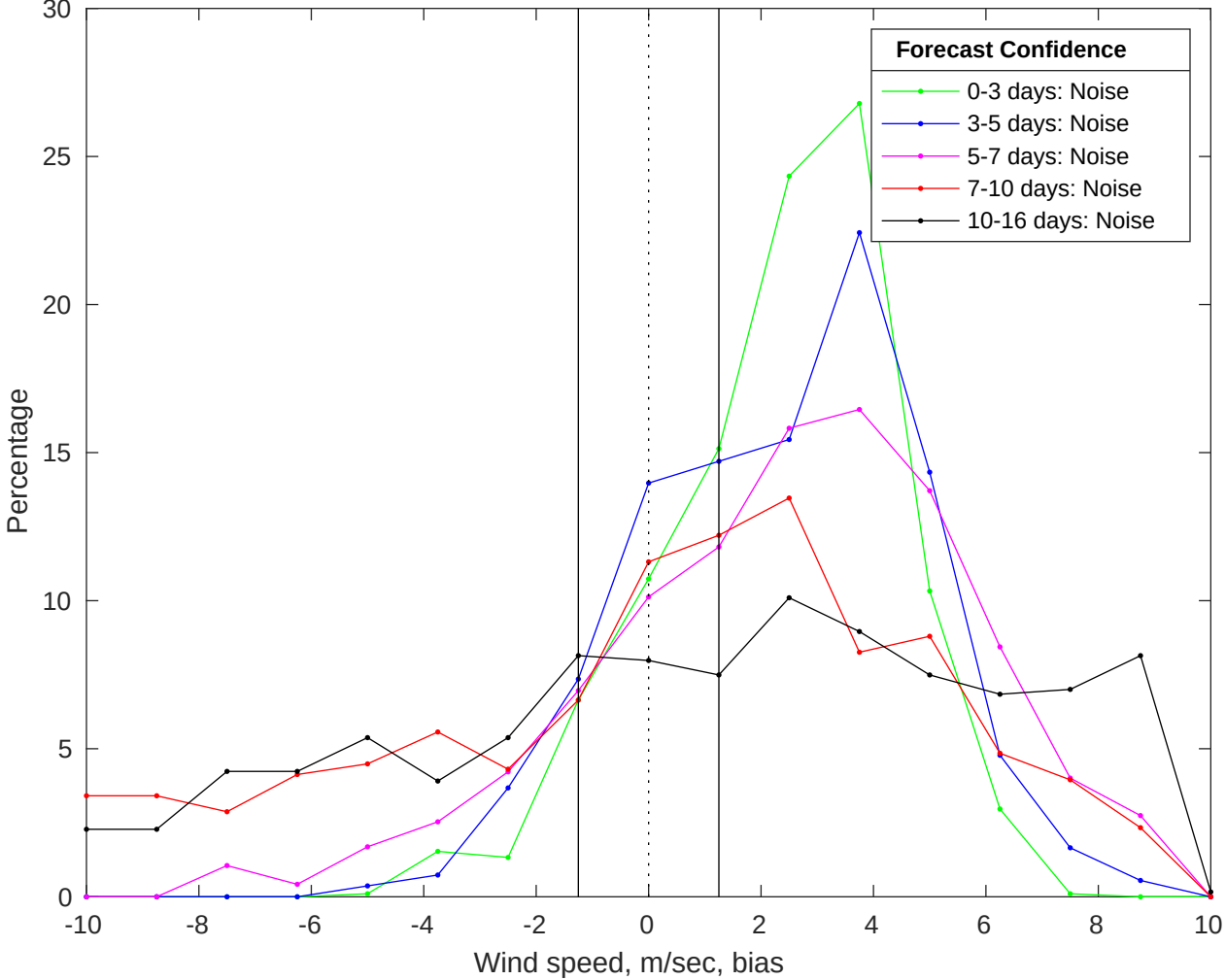
NDBC 46028 vs GFS Winds Bias Histogram: 07-Jul-2025
