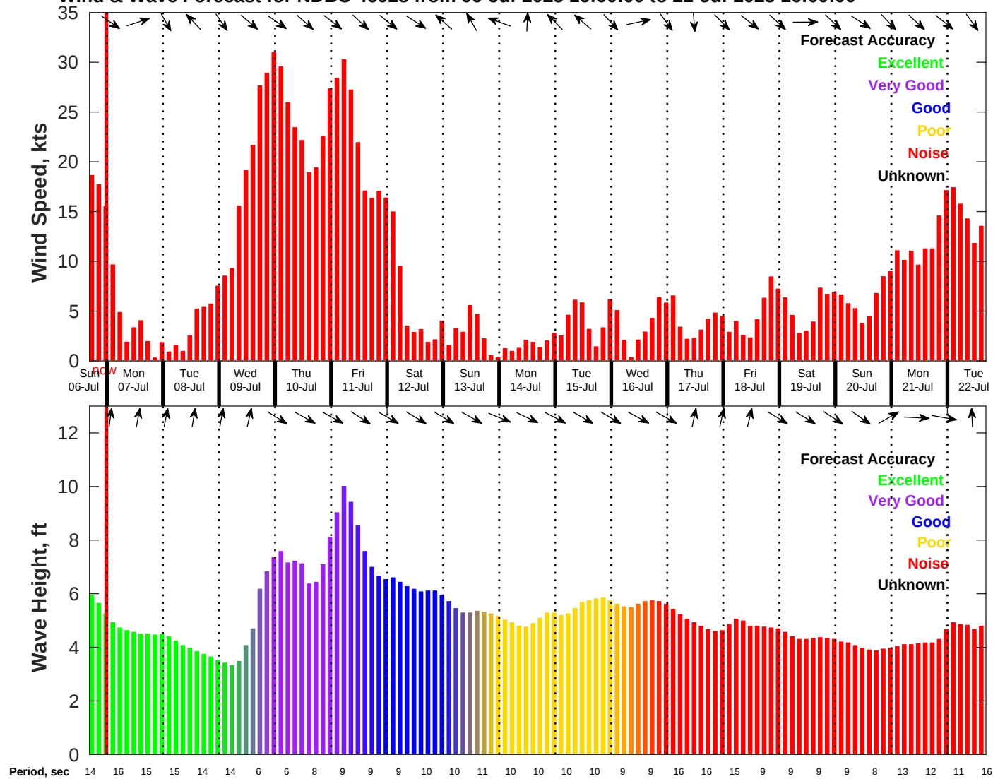
Wind & Wave Forecast for NDBC 46028 from 06-Jul-2025 16:00:00 to 22-Jul-2025 16:00:00
