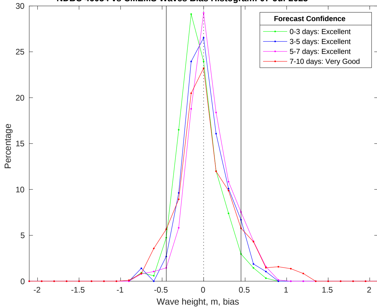
NDBC 46054 vs CMEMS Waves Bias Histogram: 07-Jul-2025
