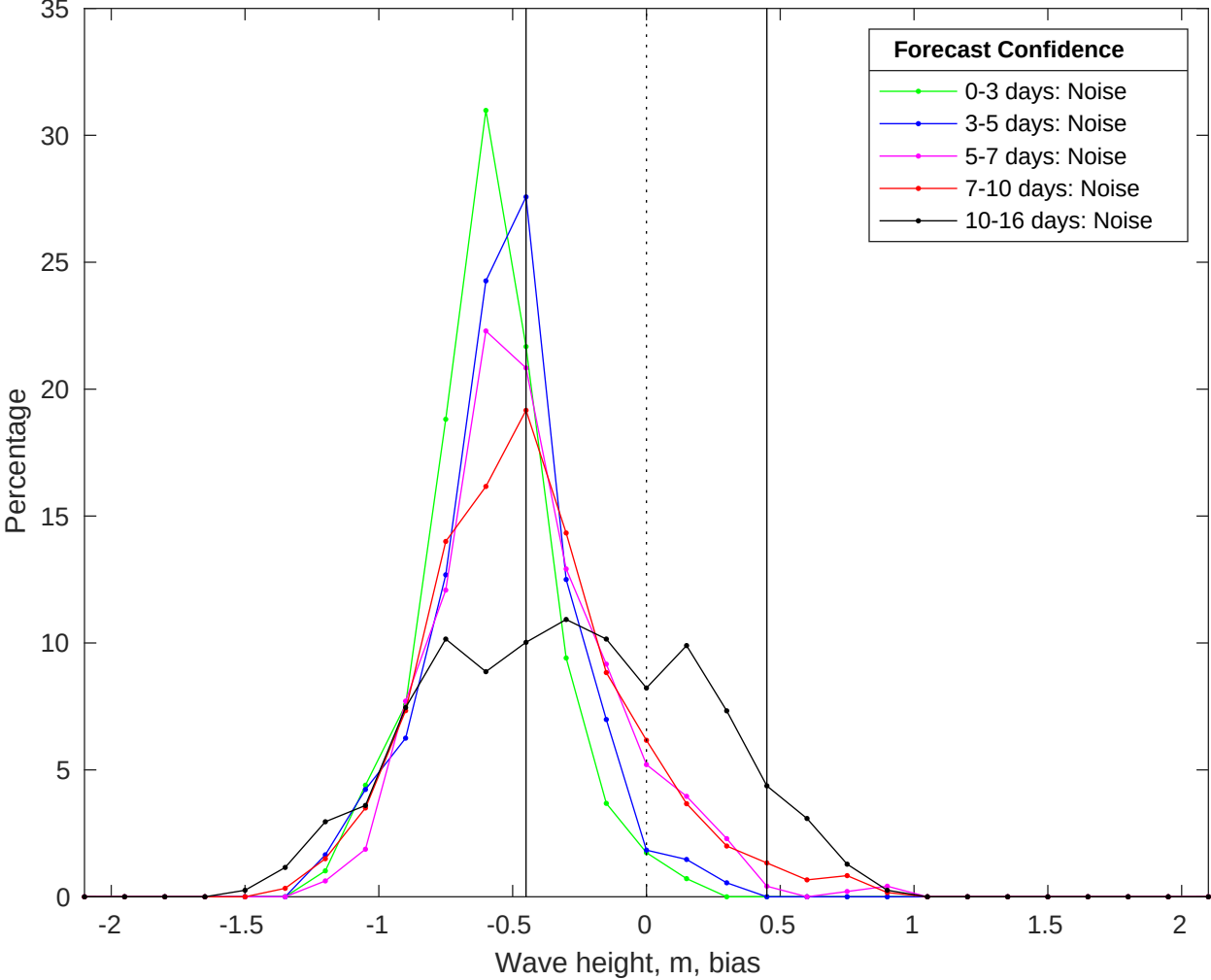
NDBC 46054 vs GFS Waves Bias Histogram: 07-Jul-2025
