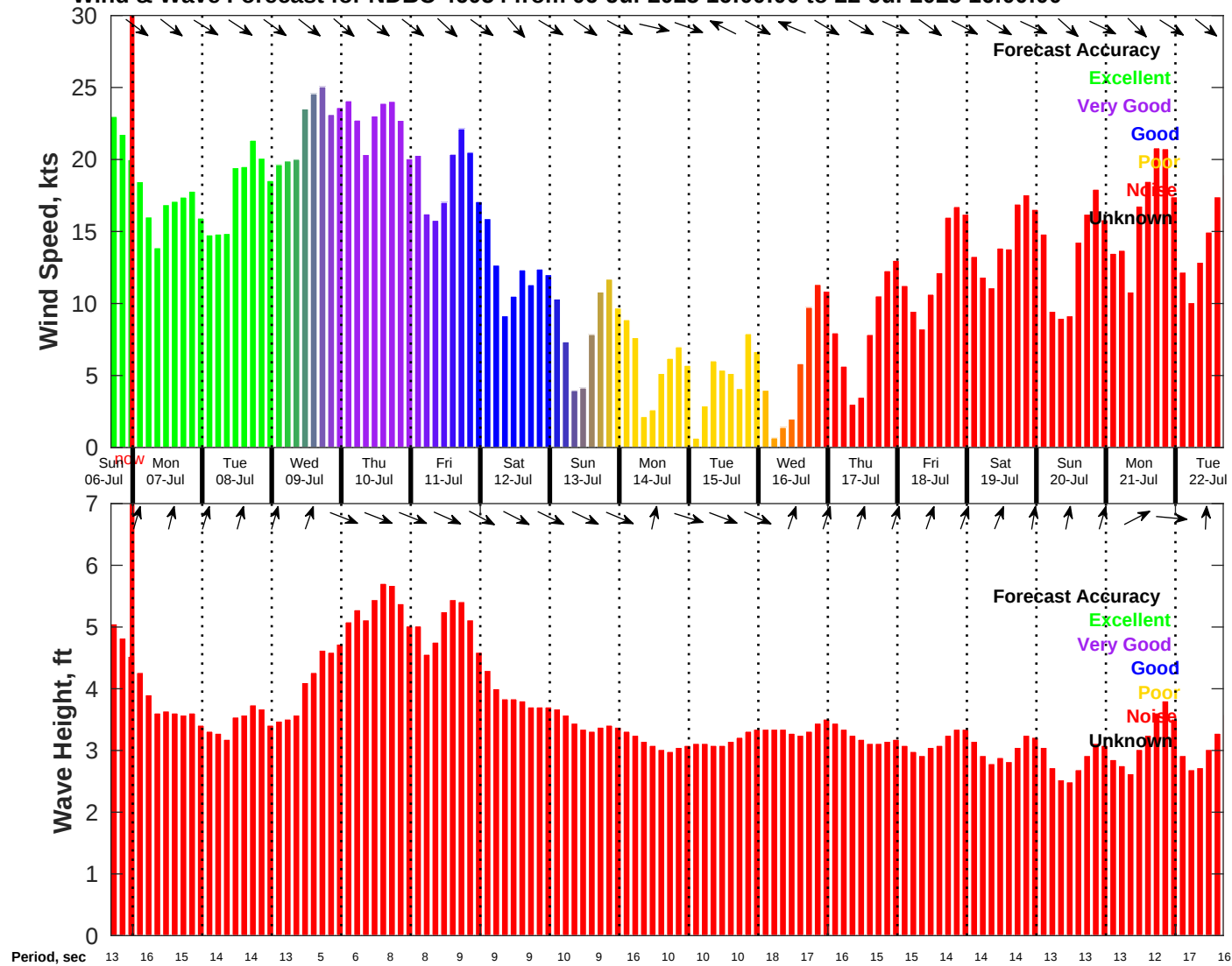
Wind & Wave Forecast for NDBC 46054 from 06-Jul-2025 16:00:00 to 22-Jul-2025 16:00:00
