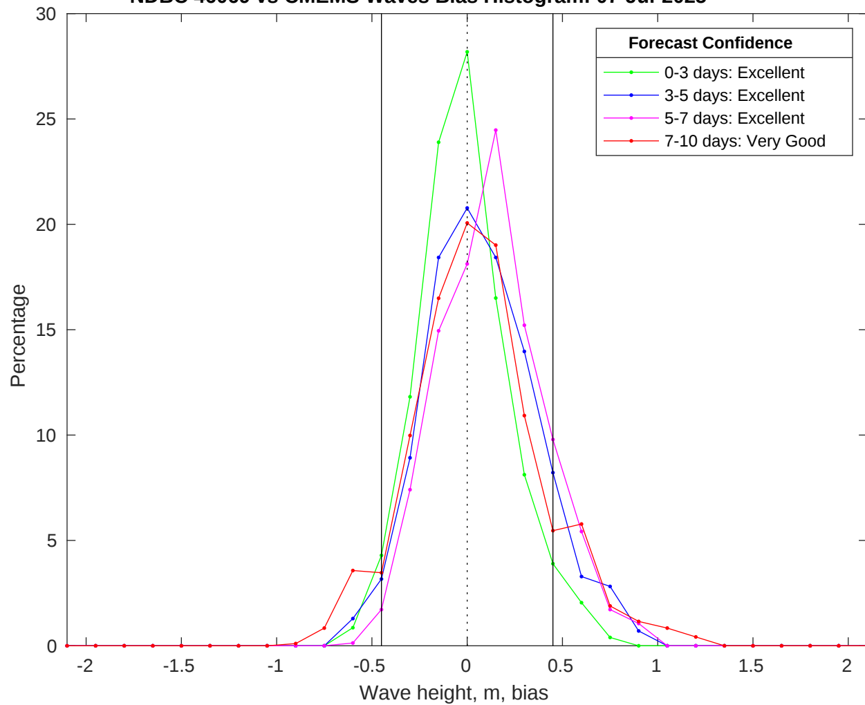
NDBC 46069 vs CMEMS Waves Bias Histogram: 07-Jul-2025
