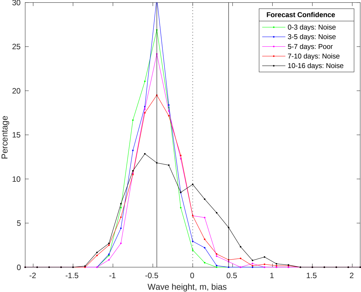
NDBC 46069 vs GFS Waves Bias Histogram: 07-Jul-2025
